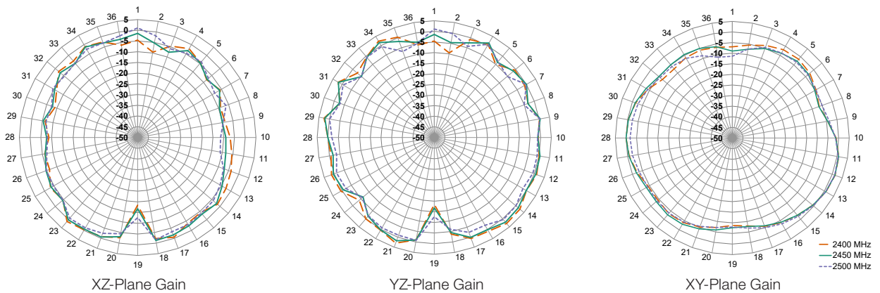
Figure 7. Radiation Patterns for ANT-2.4-FPC-SF Antenna
