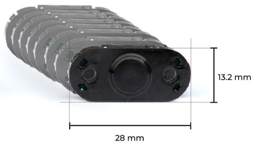
Sensors (8 units)
