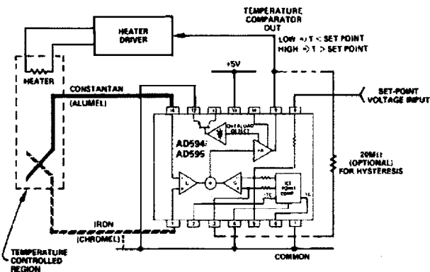
Figure 9. Set-Point Controller
