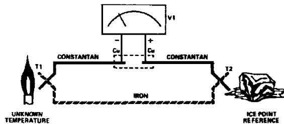
Figure 14. Thermocouple Voltage with 0^{\circ}\text{C} Reference
