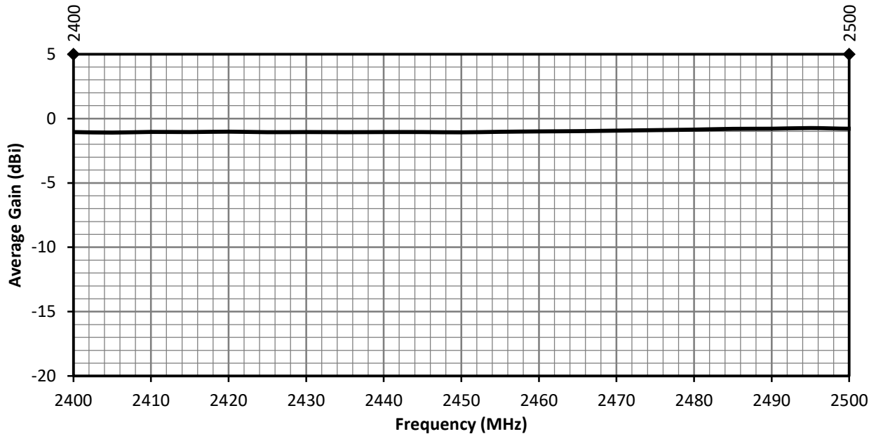
Figure 7. ANT-2.4-WRT-MON Antenna Average Gain
