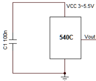
Figure 7 Typical circuit1
