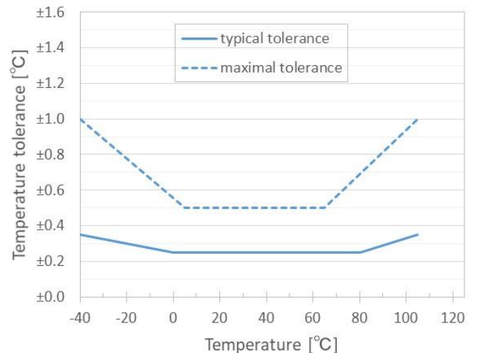
Fig.7 Temperature tolerance
