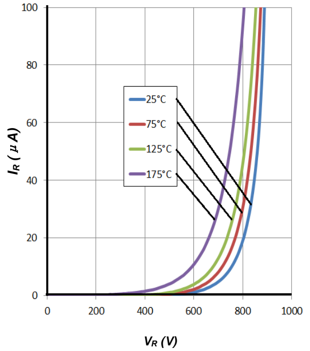
Figure 2. Reverse Characteristics
