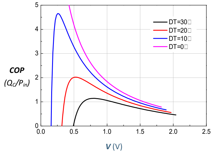
Performance Curves @ T_H = 50^\circ\text{C}
