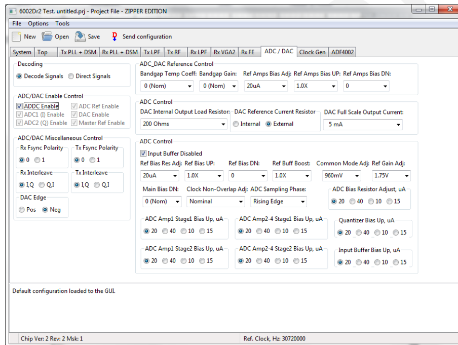
Figure 24. ADC/DAC window
