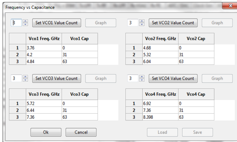
Figure 16. Frequency versus capacitance calibration table data
