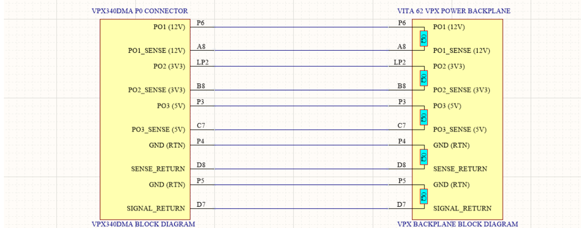
Figure 1.1: Block Diagram of VPX340DMA and VITA 62 Power Backplane. VPX340DMA requires PO1_SENSE, PO2_SENSE, PO3_SENSE, SENSE_RETURN, & SIGNAL_RETURN to be terminated on the VITA 62 Power Backplane . Verify that these connections are made on your VPX Power Backplane .
