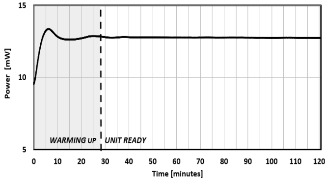
FIG. 7: WARM-UP TIME
