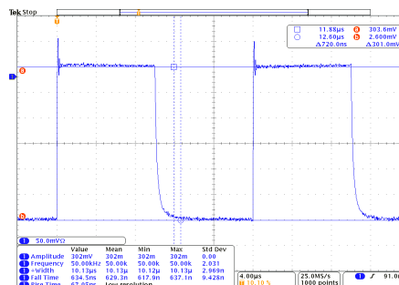
50 kHz, 10 \mu s Pulse Width, 60 A Output
