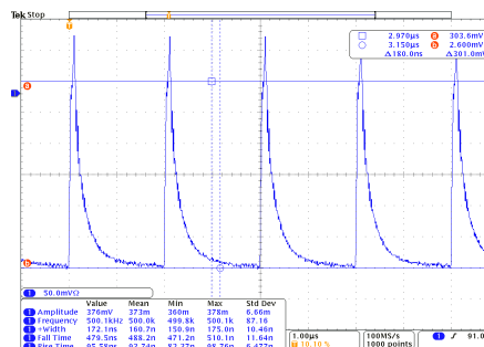
500 KHz, 172 ns Pulse Width, 60 A Output
